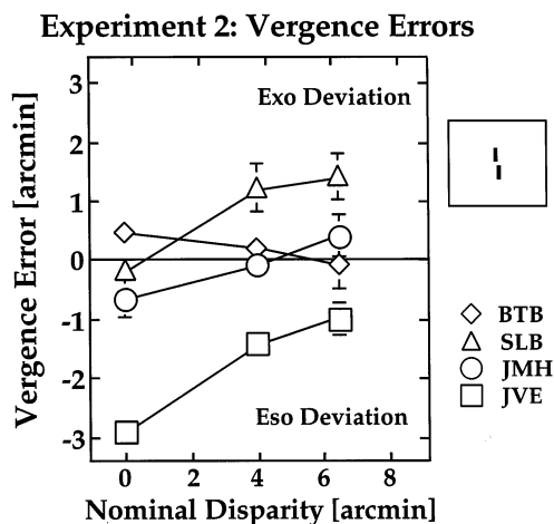
Fig. 6. Experiment 2: vergence errors during the experiment. The difference between the vergence of the fixation symbol and the actual vergence of the eyes is plotted as a function of the disparity of the fixation symbol relative to the alignment probe. The vergence of the eyes was assessed using a flashed fixation–disparity probe (see text for details). If vergence were precise, the data would lie on the horizontal line at 0. The data points represent the estimated vergence errors for the four observers. Exo-deviations (i.e. the eyes verged behind the fixation symbol) are indicated by points above the horizontal line at 0 and eso-deviations (i.e., the eyes verged in front of the symbol) are indicated by points below. Error bars represent \pm 1 S.D. These data were used to correct the alignment data (see Fig. 8) for vergence errors.
