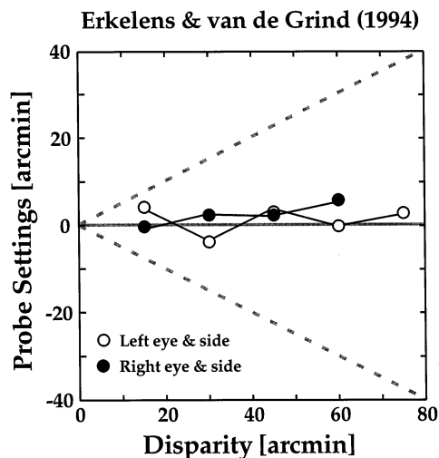
Fig. 12. Probe settings of observer CE in Erkelens and van de Grind (1994) as a function of the probe's disparity relative to the fixation point. The dashed gray lines represent Hering's predictions and the solid gray lines Erkelens' predictions.
