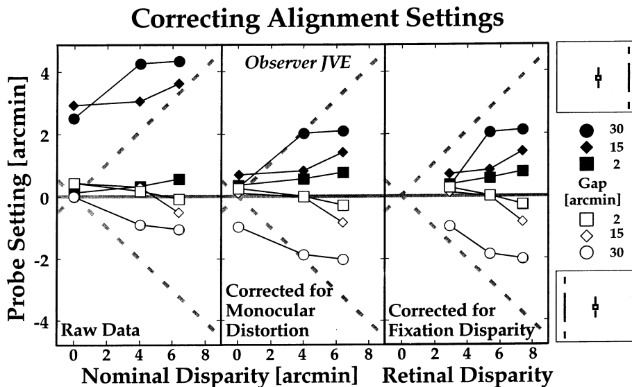
Fig. 8. Alignment settings and corrections for vergence errors and monocular distortion. The left panel shows the data from observer JVE; the data are the same as in the right panel of Fig. 5. The azimuth of the alignment probe setting relative to the standard line is plotted as a function of the disparity of the fixation symbols relative to the alignment probe. The central panel shows the same data once corrected for the monocular distortions measured in Experiment 3 (see Fig. 7). These errors are corrected by shifting the data at each gap size vertically in order to undo the azimuthal distortion observed in Experiment 3. The right panel shows the data from the central panel once corrected for the vergence errors measured in Experiment 2 (see Fig. 6). These errors are corrected by plotting the retinal disparity on the abscissa rather than the nominal disparity.
