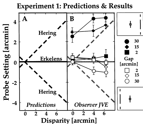
Fig. 5. Predictions and results for Experiment 1. (A) Hering's and Erkelens' predictions. The azimuth of the predicted probe setting relative to the standard line is plotted as a function of its disparity relative to the fixation point; azimuths are calculated for the eye that sees both the alignment probe and the standard line. Erkelens' prediction is that the probe should be set to the same azimuth as the standard line; thus, the prediction is 0 for all disparities. Hering's prediction is that the probe's azimuth relative to the standard line should be half its disparity. The predictions are the dashed diagonal lines; the upper and lower lines are the prediction when the standard line is to the left and right of fixation, respectively. (B) The probe settings of observer JVE are plotted in the same format. The gray lines represent the predictions. The filled symbols represent the settings when the standard line was to the left of fixation and the unfilled symbols the settings when the standard line was to the right. The squares, diamonds, and circles represent data for gap sizes of 2, 15, and 30 arcmin, respectively. Error bars represent \pm 1 S.D.
