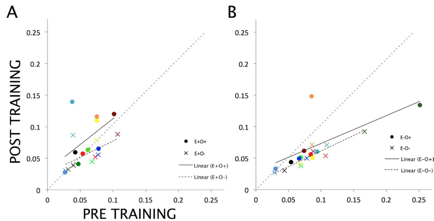
Figure 2. Pre- and post-training contrast detection thresholds. (A) Detection thresholds of all 10 observers for the eye in which the grating was presented during training, both for the trained ( E+O+ ) and for the untrained orientation ( E+O- ). (B) Detection thresholds for the same 10 observers, but now for the eye in which the grating was not presented during training, again both for the trained ( E-O+ ) and for the untrained orientation ( E-O- ). Data points are color-coded consistently within observers. Data points below the diagonal dashed line indicate better performance (i.e., lower thresholds) after training than before training, while data points above this line indicate worse performance after training (i.e., higher thresholds). Linear regression lines are added for all conditions.
