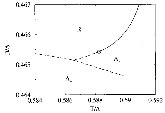
Fig. 10. Detail of a phase diagram in regime 5 ( \Delta = 1.4, \epsilon = 0.01 ). Solid and dashed lines mark second and first order transitions, respectively; circles indicate tricritical points. There is a three-phase point where the three first order lines meet.
