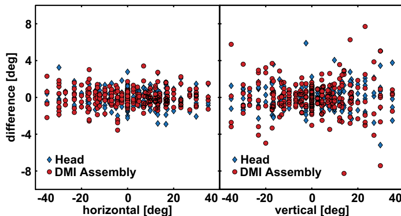
FIG. 5. Difference of calibrated mean endpoint of a given target and 4 repetitions made to the same target as a function of horizontal (left) and vertical (right) target position for V_{net} of the DMI assembly (red circles) and the head coil (blue diamonds). Subject PB.
