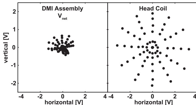
FIG. 4. Uncalibrated endpoints for the DMI assembly ( V_{net} ) (left column) and the head coil (right column) for subject PB. Note that an ideal DMI assembly would yield a V_{net} of zero for all head orientations. Here, the vertical endpoints for the DMI assembly are strongly compressed in the lower hemisphere.
